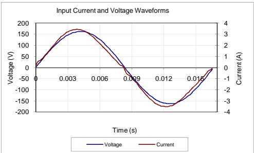
Input AC Current Waveform (ITHD = 5.92%, 50% Load)
